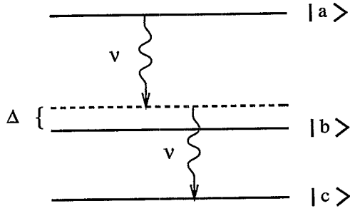
FIG. 1. Level scheme for the two-photon correlated-spontaneous-emission laser. The atoms are pumped into a coherent superposition of states |a\rangle and |c\rangle , with no population in the relay level b .
