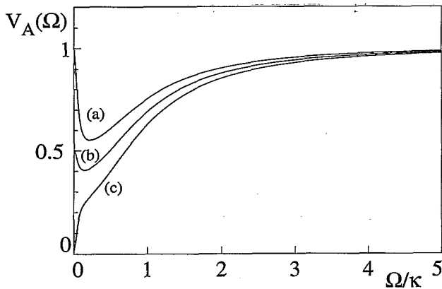
FIG. 3. Normalized spectrum of amplitude fluctuations for a laser of the third class for different statistical parameters p . (a) p = 0 (Poissonian pumping), (b) p = 0.5 (intermediate case), (c) p = 1 (regular pumping). High-above-threshold operation, r = 10^6 . For all curves a' = 0 , a = 0.001 , b = 0.1 .
