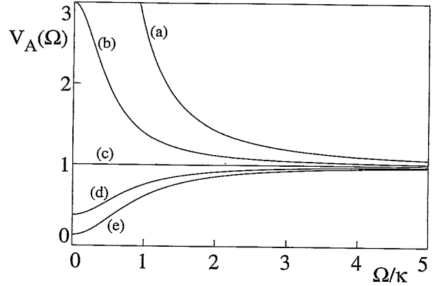
FIG. 2. Normalized spectrum of amplitude fluctuations for a laser of the first class for several pump parameters r . (a) r = 1.1 , (b) r = 2 , (c) r = 3 , (d) r = 5 , and (e) r = 10 . For all curves a' = a = 0 , p = 1 .
