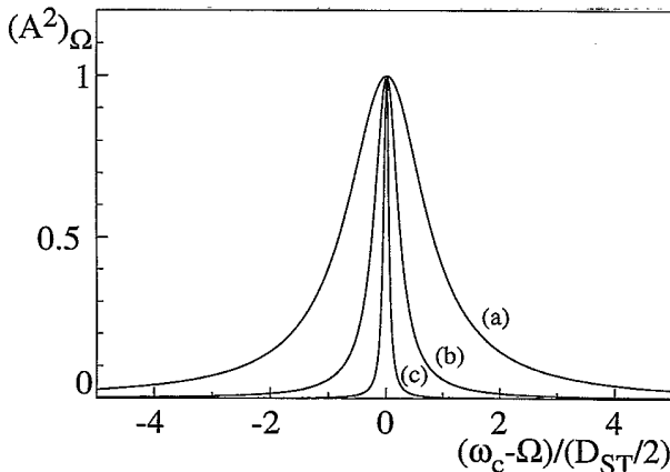
FIG. 1. Normalized power spectrum of the laser with atomic-memory effect. For all three curves D_{ST}/\kappa = 10^{-10} . (a) 2\gamma_{ab}/\kappa = 10 , i.e., Schawlow-Townes limit, (b) 2\gamma_{ab}/\kappa = 1 , and (c) 2\gamma_{ab}/\kappa = 0.3 (long-lived atomic polarization).
