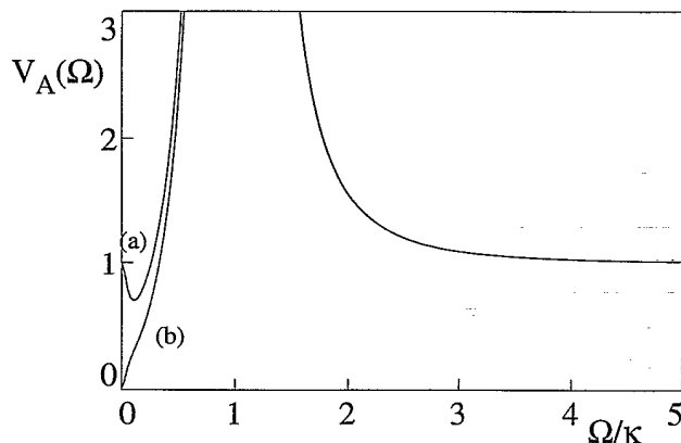
FIG. 6. Normalized spectrum of amplitude fluctuations for a laser of the fourth class for Poissonian pumping, p = 0 [curve (a)] and regular pumping, p = 1 [curve (b)]. For both curves a' = 0 , a = 0.001 , b = 0.1 , c = 0.5 ; r = 10^3 .
