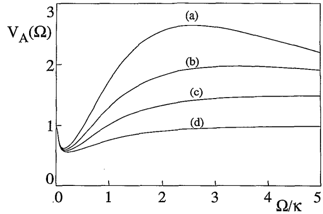
FIG. 4. Normalized spectrum of amplitude fluctuations for a laser of the third class for Poissonian pumping, p = 0 , and different pump parameters r . (a) r = 3 \times 10^3 , (b) r = 5 \times 10^3 , (c) r = 10^4 , and (d) r = 10^6 . For all curves a' = 0 , a = 0.001 , b = 0.1 .
