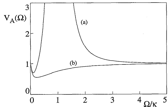
FIG. 5. Normalized spectrum of amplitude fluctuations for a laser of the fourth class for Poissonian pumping, p = 0 , and different pump parameters r . (a) r = 10^3 , (b) r = 10^6 . For both curves a' = 0 , a = 0.001 , b = 0.1 , c = 0.5 .
